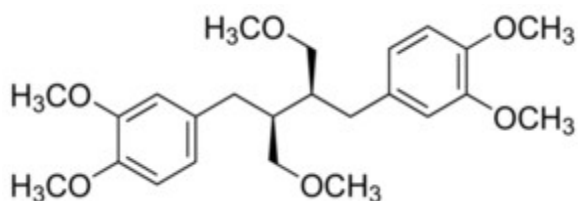
Phyllanthin
