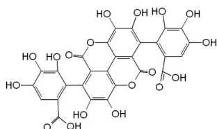
Gallagic acid
