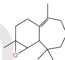
\beta himachalene
