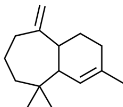
\alpha -himachalene
