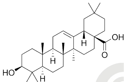
Oleanolic acid
