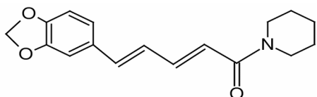
Piperine
