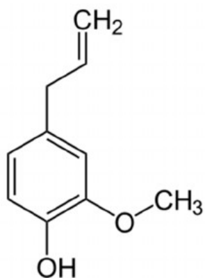
Eugenol
